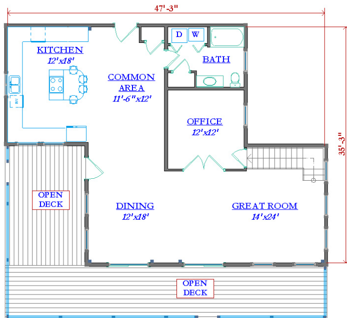
HOLBROOK 2210 Sq. Ft.
